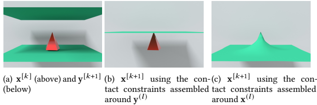
Fig. 3. Linearization choices. The tunneling artifact occurs between two intersection-free states \mathbf{x}^{[k]} and \mathbf{y}^{[k+1]} (Fig. (a)). Projecting \mathbf{y}^{[k+1]} back to \Omega based on the constraints assembled around \mathbf{y}^{(l)} stagnates \mathbf{x}^{[k+1]} (Fig. (b)). Instead, if we assemble and linearize contact constraints around \mathbf{x}^{(l)} , \mathbf{y}^{(l)} manages to cross the boundary of \Omega and stay on the same side as \mathbf{x}^{(l)} , eventually advancing \mathbf{x}^{(l)} to a more reasonable solution (Fig. (c)).
