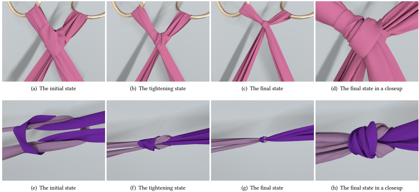
Fig. 1. Knotting. The bow knot example (on the top, with 142K triangles) and the reef knot example (on the bottom, with 71K triangles) are presented. In this work, we develop a two-way method for safe and fast collision handling in deformable body simulation. Thanks to this method, our simulator can robustly handle complex collision contacts in these two examples at 4 to 17 FPS and 10 to 21 FPS respectively.
