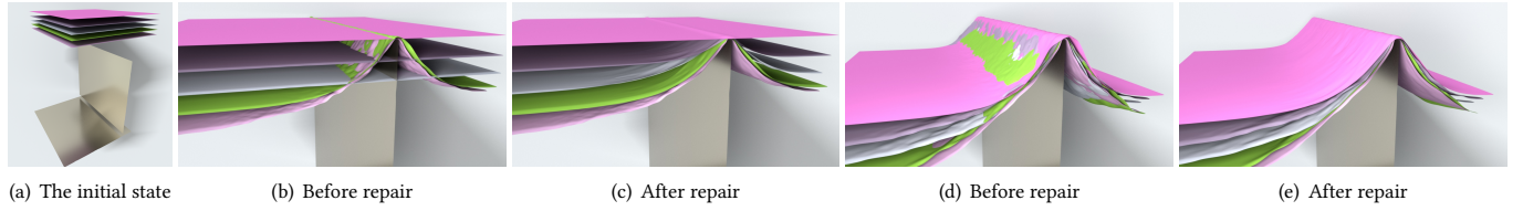
Fig. 15. Cloth and blade colliding. In this example, five square cloth patches are dropped onto a sharp metal blade, and then they drape, slide and stack under gravity. Our method reliably projects severely penetrated frames ((b) and (d)) to intersection-free states ((c) and (e)).
