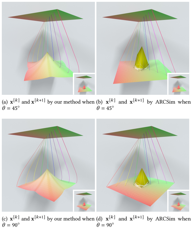
Fig. 18. Trajectories avoiding collisions. Here, we track the trajectories of nine vertices along one diagonal of the cloth patch, which are generated progressively using our two-way approach. Compared to the impact zone optimization implemented by ARCSim [Narain et al. 2012], our method enables a curved path from \mathbf{x}^{[k]} to \mathbf{x}^{[k+1]} to resolve collisions without the occurrence of intersections or spuriously stretched elements, while limiting the path to a linear trajectory may fail to find a faithful solution at a reasonable cost.
